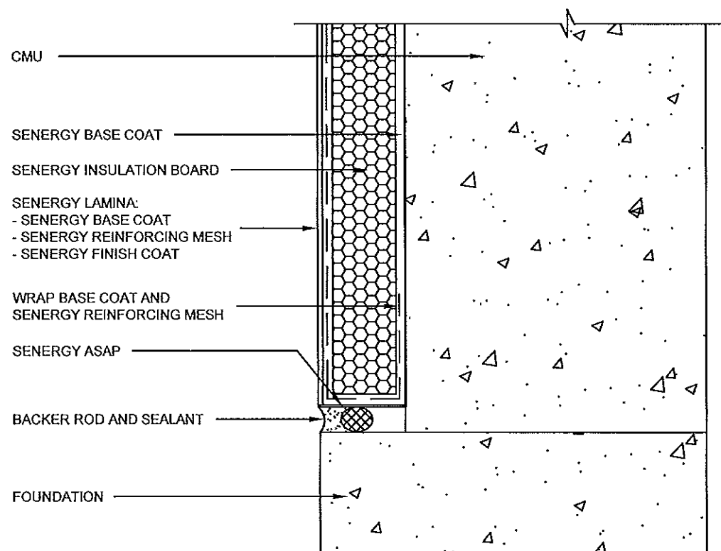
TYPICAL TERMINATION AT FOUNDATION (FLUSH)
