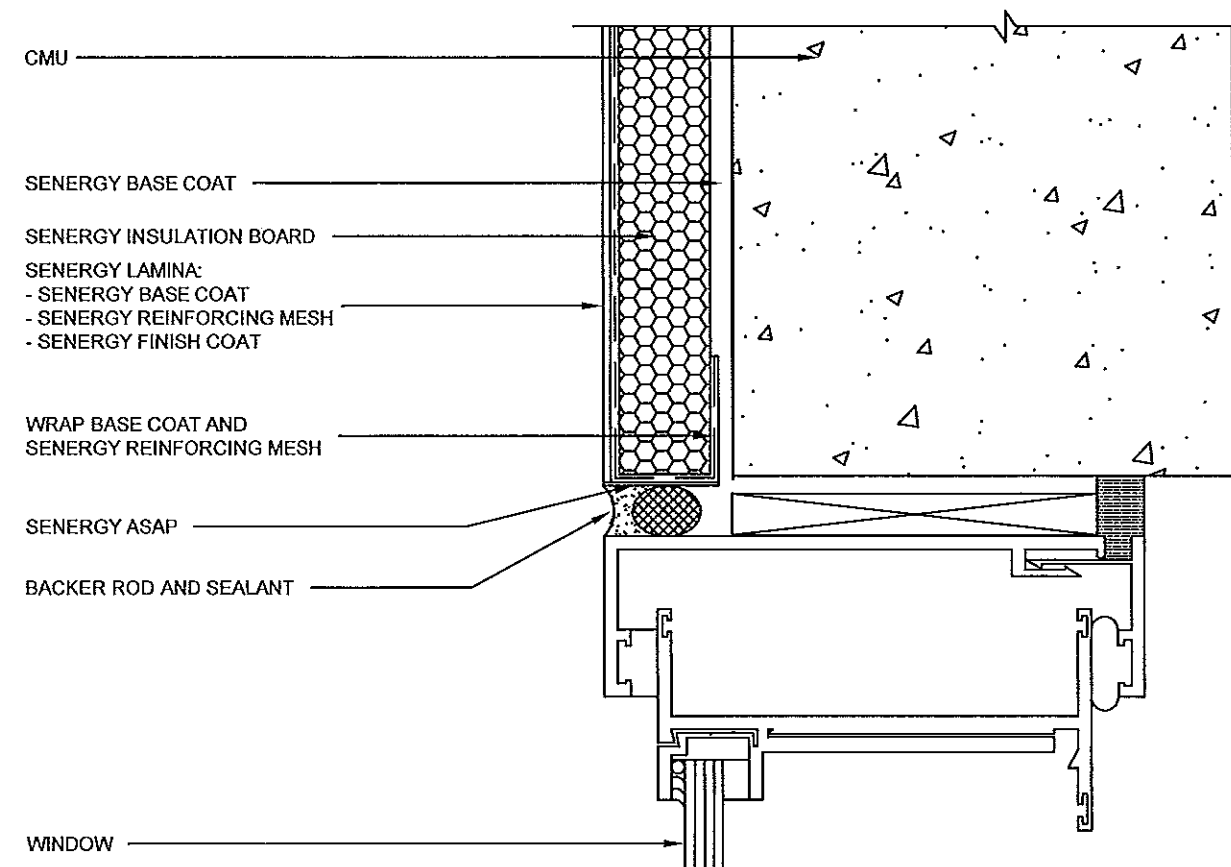
TYPICAL WINDOW JAMB (FLUSH)
