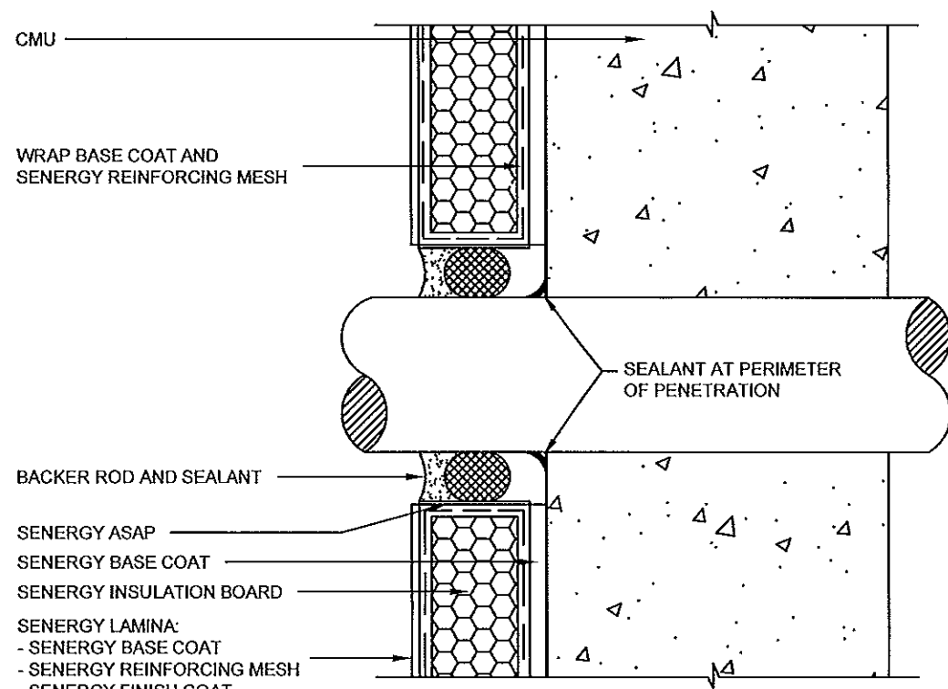
TYPICAL PIPE PENETRATION
