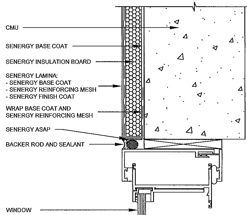
TYPICAL WINDOW HEAD (FLUSH)
