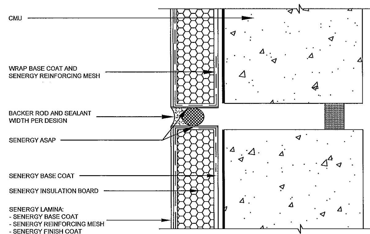
TYPICAL EXPANSION JOINT
